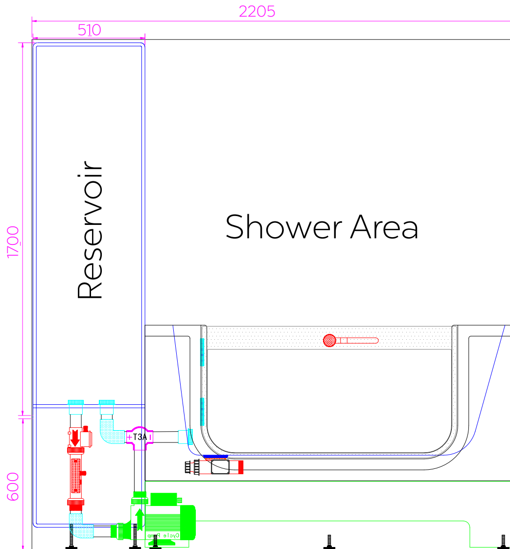
400L Water Tank with Lay Down Tub LD6632 FRONT VIEW
